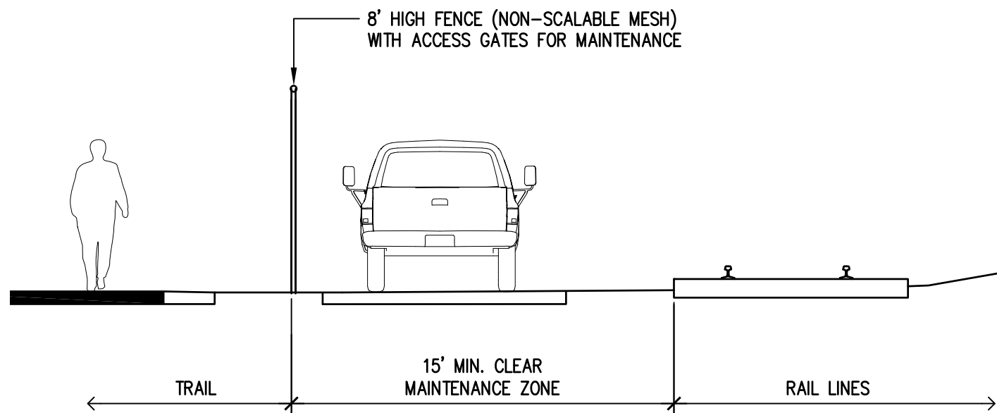
Figure 1.5: Minimum Clear Zone and Separation Fence
