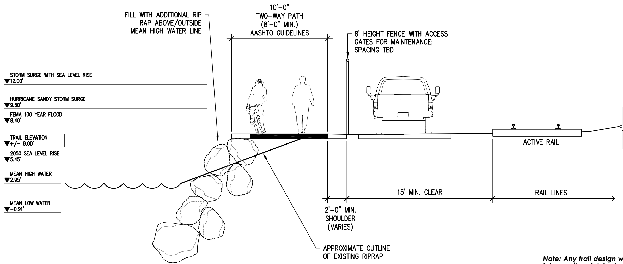
FIGURE 2.4: TYPE 2 TRAIL- BUILT-UP RIP-RAP
