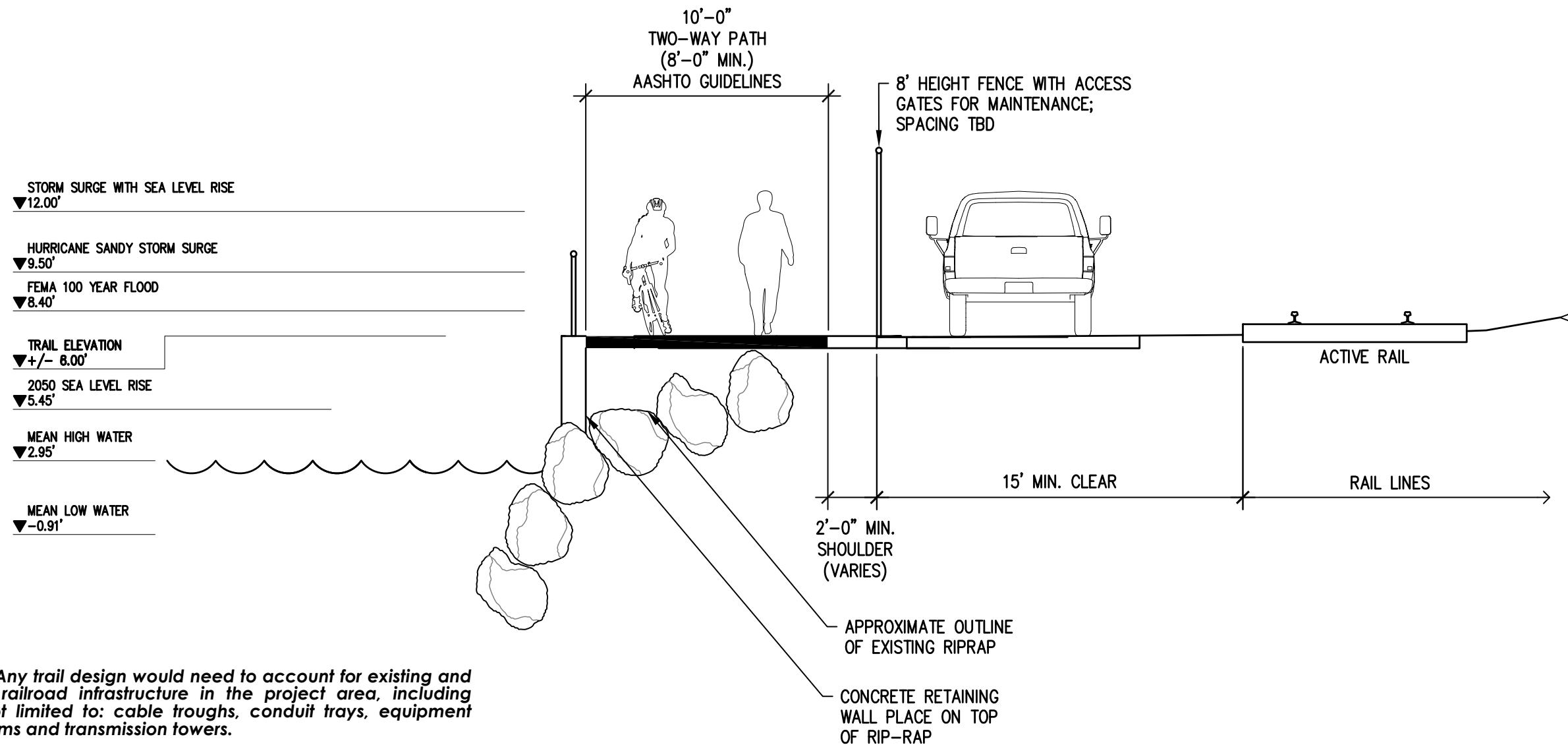
FIGURE 2.5: TYPE 3 TRAIL - RETAINING WALL
