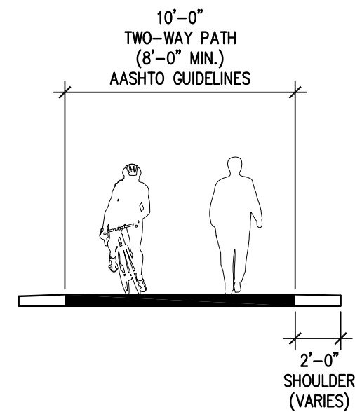
Figure 1.6: Minimum Trail Width
